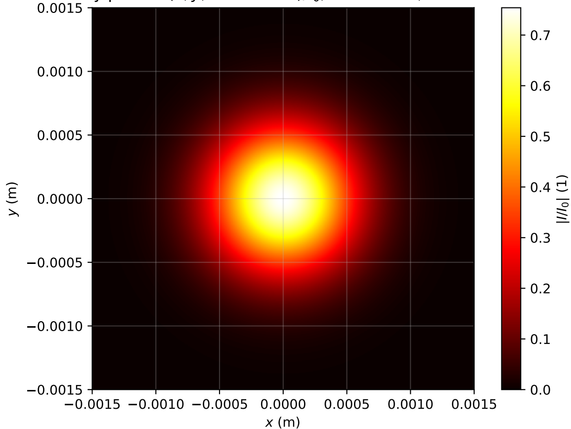
Intensity profile I(x, y, z = 1.274m)/I_0 , Pin=0.1Pcr, artificial time
